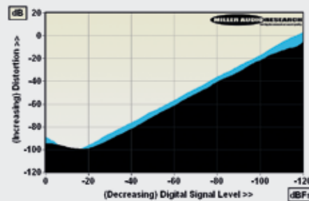
ABOVE: THD versus 16-bit CD digital signal level over a 120dB range at 1kHz (black) and 20kHz (blue)
