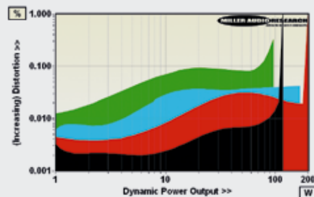
ABOVE: Dynamic power output versus distortion into 8ohm (black trace), 4ohm (red), 2ohm (blue) and 1ohm (green) speaker loads. Max. current is 9.8A
